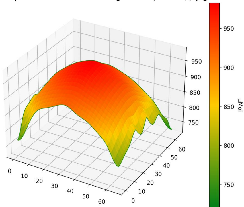
PPFD 3D Heatmap LT-5949 - 3500K - Distance @ 115cm - power supply @ 100%
